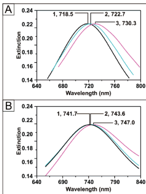
Figure 2. Demonstration of the LSPR sandwich assay at high and low concentrations. (A) LSPR spectra for each step of the sandwich assay for 10 pM ADDL. Ag nanoparticles after modification with (A-1) 100 nM anti-ADDL antibody, \lambda_{\max} = 718.5 nm, (A-2) 10 pM ADDL, \lambda_{\max} = 722.7 nm, and (A-3) 100 nM anti-ADDL, \lambda_{\max} = 730.3 nm. (B) LSPR spectra for each step of the sandwich assay for 100 fM ADDL. Ag nanoparticles after modification with (B-1) 100 nM anti-ADDL antibody, \lambda_{\max} = 741.7 nm, (B-2) 100 fM ADDL, \lambda_{\max} = 743.6 nm, and (B-3) 100 nM anti-ADDL, \lambda_{\max} = 747.0 nm. All spectra were collected in N_2 .
